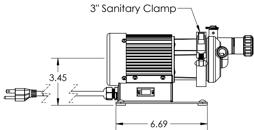
Right View
